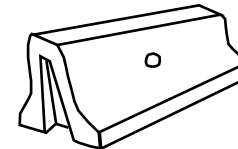
CTB-1 Concrete Transition Barrier 690mm > 457mm x 2.5m 2700 lbs Female only
