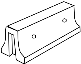
CMB Concrete Median Barrier 810mm x 2.5 m 3800 lbs CMB-M (Male) 1.0" Hook CMB-F (Female)
